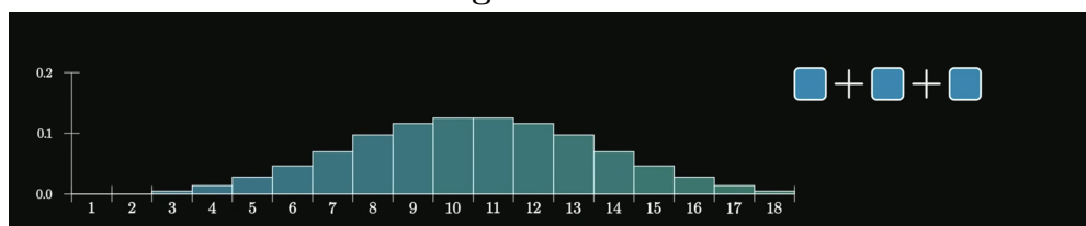
Figure 4. n=3
