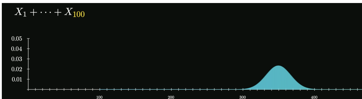
Figure 6. n=100
