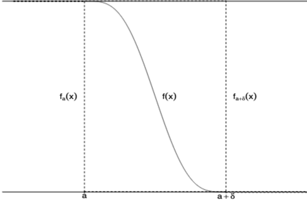
Figure 11. Sandwiching the smooth function
