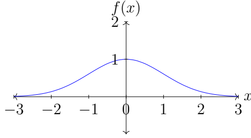
Figure 1. The standard normal distribution
