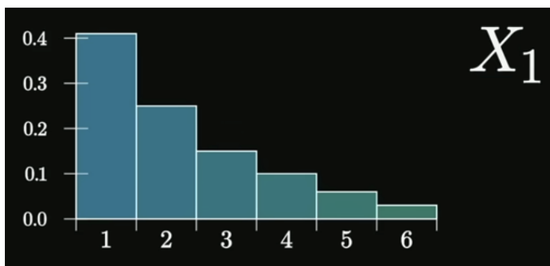
Figure 7. unfair die
