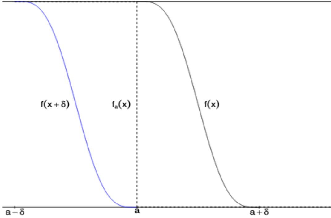
Figure 12. Sandwiching f_a(x)
